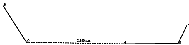
Figure 1. SCF-optimized geometry of the water-ion dimer.
